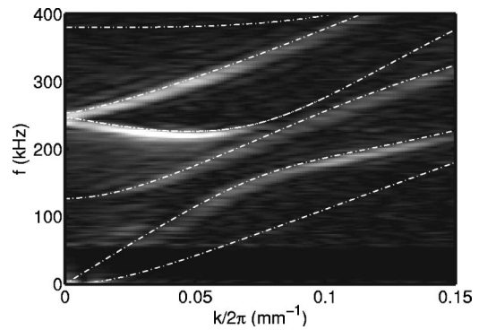
FIG. 3. Measured dispersion spectrum of 5.46-mm Lucite, with the calculated dispersion curves of Fig. 1 overlaid.
