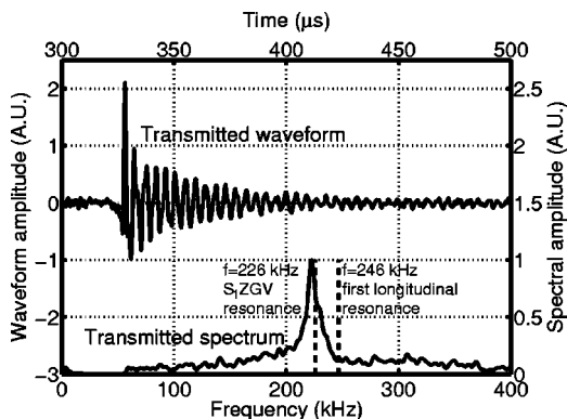
FIG. 2. Wave form and spectrum of ultrasound transmitted through 5.46-mm Lucite.
