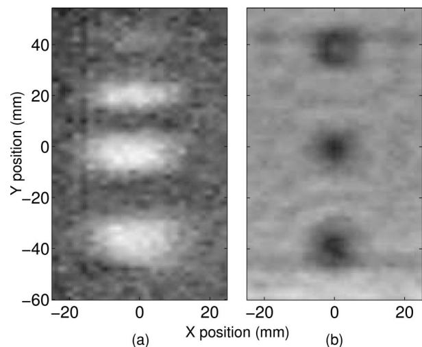
FIG. 4. (a) Air-coupled C-scan image of Scotch-tape strips on Lucite, 218 kHz, (b) Air-coupled C-scan image of Teflon inserts buried within carbon fiber epoxy, 186 kHz.
