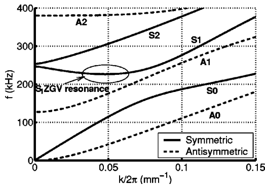
FIG. 1. Dispersion relation of Lamb modes for Lucite, calculated from theory and nominal elastic parameters ( C_{11}=8.6 GPa, C_{12}=4.1 GPa, \rho = 1191 kg/m 3 ).
