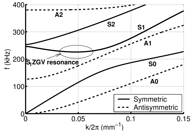
FIGURE 1. Calculated dispersion relation for 5.46-mm Lucite.
