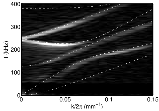
FIGURE 2. Measured transmission dispersion spectrum for 5.46-mm Lucite.
