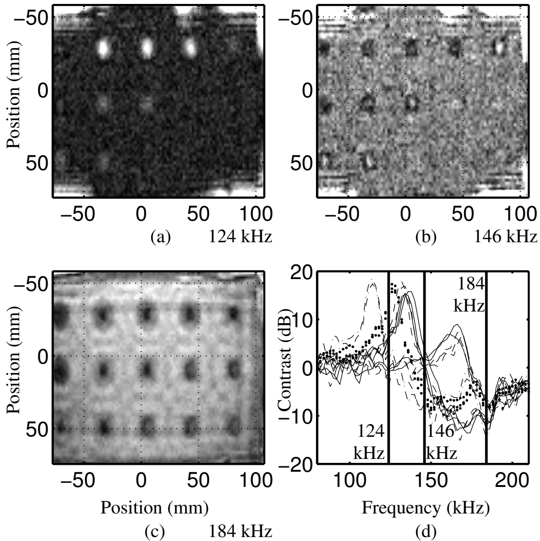
FIGURE 7. (a) 124 kHz transmission C-scan of 8.1-mm carbon fiber epoxy laminate with 3.2-6.4 mm diameter Teflon inclusions. (b) 146 kHz C-scan. (c) 184 kHz S 1 ZGV C-scan. (d) Contrast of the different inclusions as a function of frequency. Different line styles indicate different inclusion size and position.
